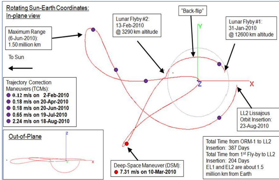
Figure 5. P1 Multi-body Trajectory Transfer
