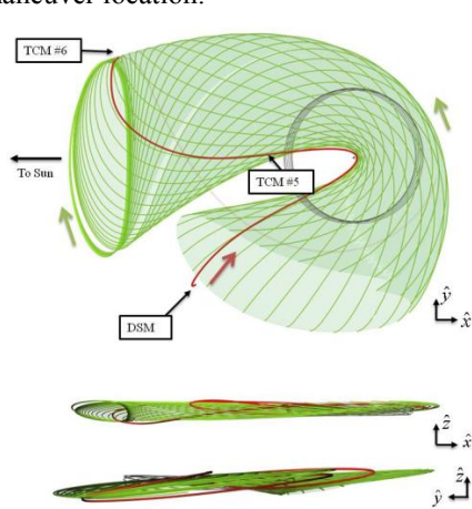
Figure 18. P1 Planned Stable Sun-Earth Earth Manifold
