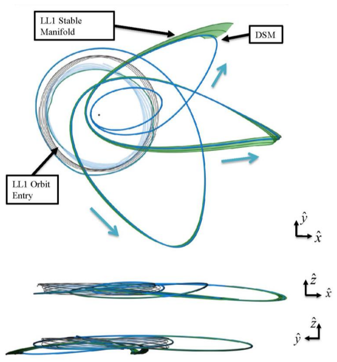
Figure 21. P2 Manifold to L_1 Lissajous Targeted State
