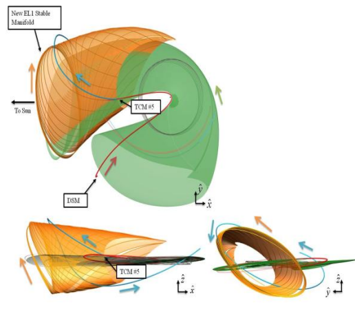
Figure 19. P1 Pre and Post TCM5 Stable Sun-Earth Manifold
