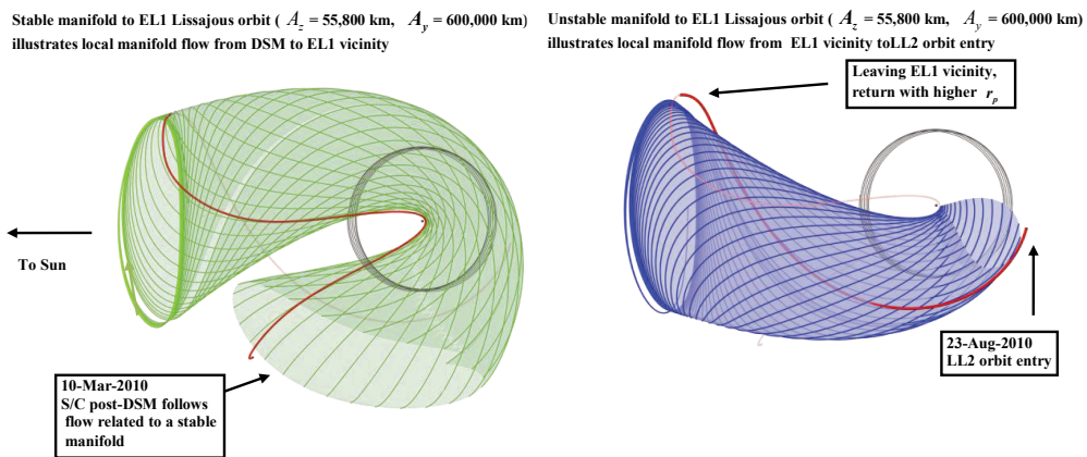
Figure 4. Baseline P1 Out-Bound to Max Radius on Stable Manifold and In-Bound to Lissajous Orbit on Unstable Manifold
