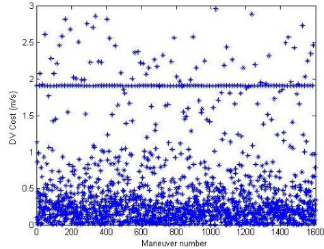
Figure 12. P1 TCM8 MC Analysis
