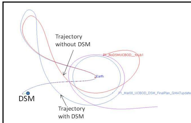
Figure 13. Preplanning and Optimized P1 DSM
