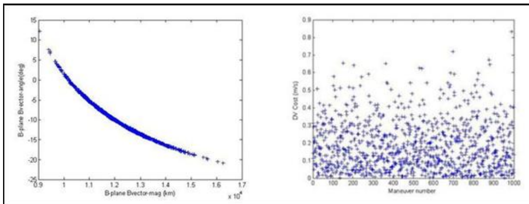
Figure 7. 2 nd Flyby B-Plane Distribution with Navigation errors
