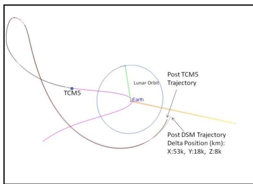
Figure 13. Preplanning and Optimized P1 DSM
