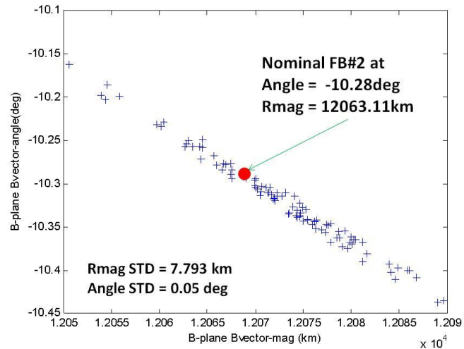
Figure 9. Post TCM4 Estimated B-plane errors
