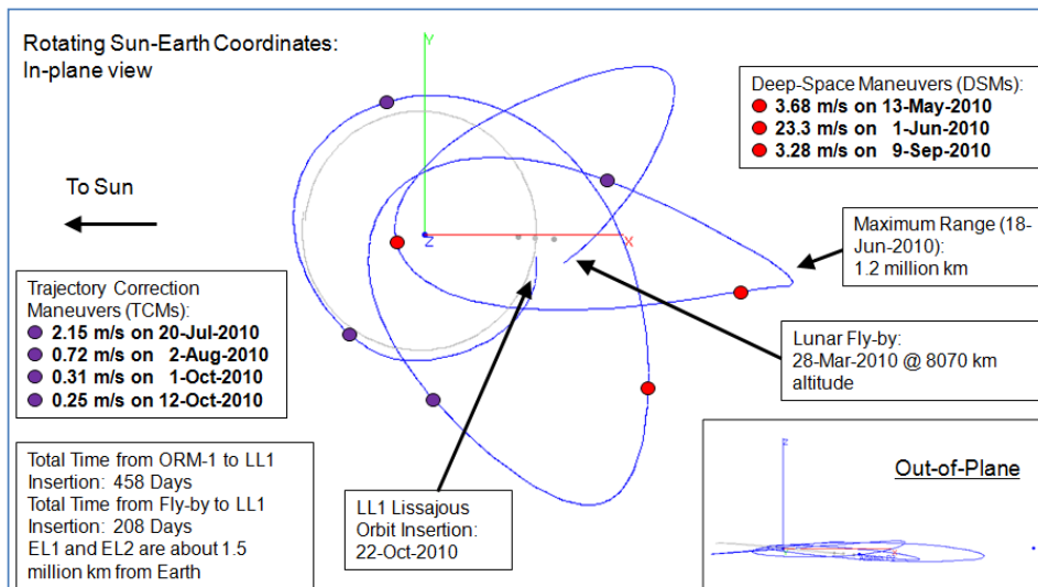
Figure 6. P2 Multi-body Trajectory Transfer
