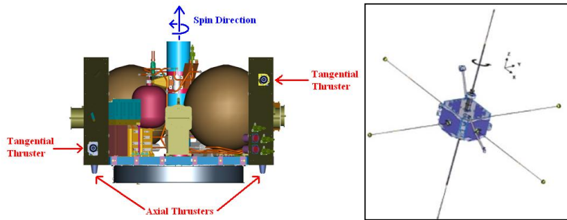
Figure 3. ARTEMIS Spacecraft Bus Design
