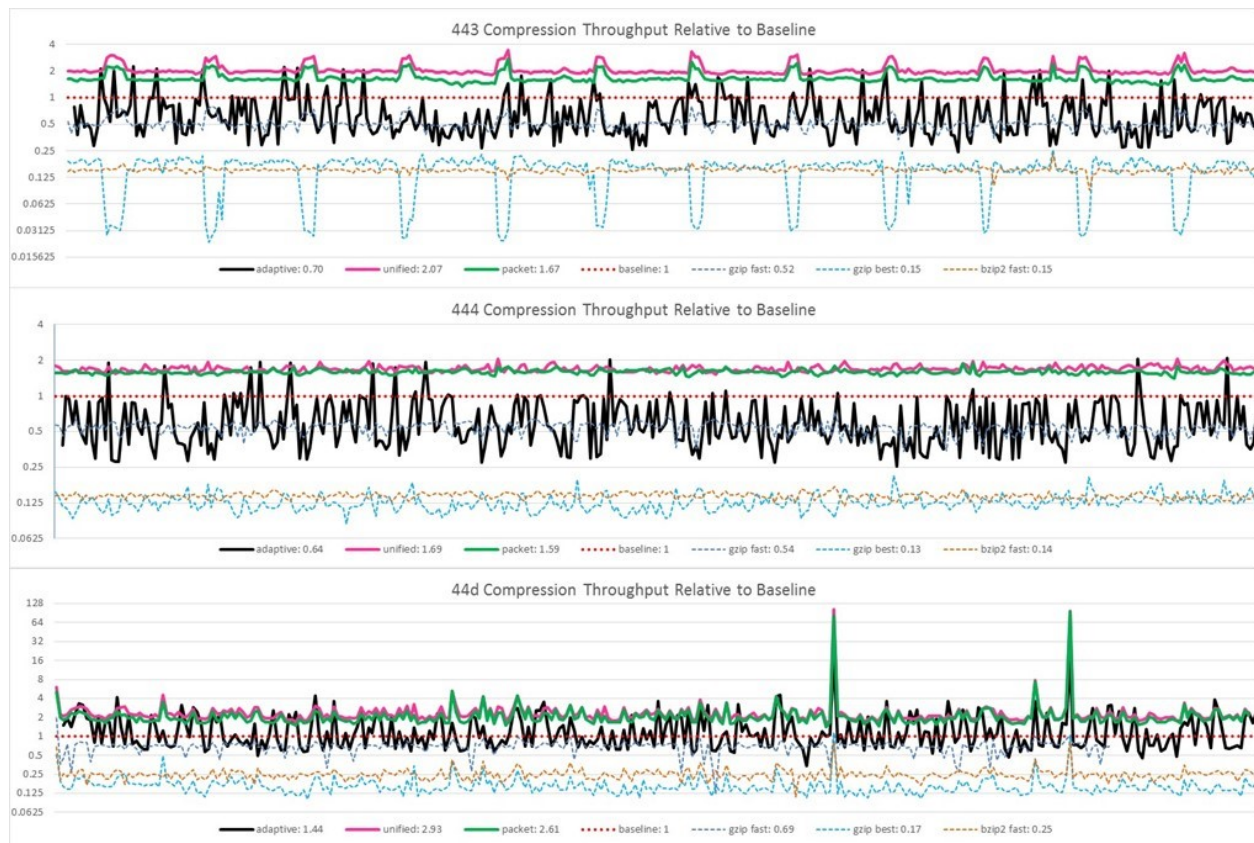
Figure 4: Daily compression throughput relative to the baseline over a year for each studied packet type
